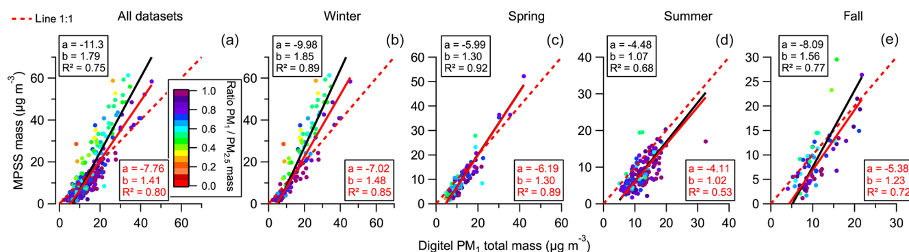
Figure 10. (a) Comparison between filter PM 1 total mass concentrations and the MPSS-derived mass concentrations for the entire period and (b–e) the different seasons. The black lines and boxes correspond to the regression fitting without threshold correction and the red lines to the regression fitting according to a PM 1 : PM 2.5 > 0.6.
