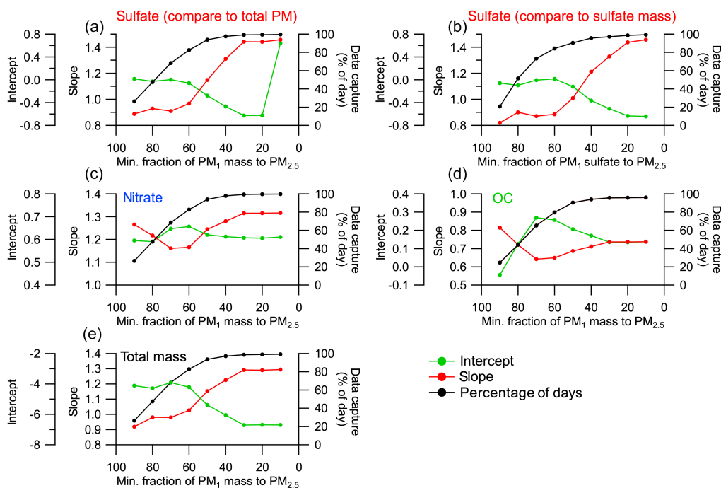
Figure 3. Sensitivity analysis of the correlation between ACSM and \text{PM}_1 sulfate, nitrate, OC, and total mass concentration depending on the \text{PM}_1 : \text{PM}_{2.5} ratio of the total mass concentration in the range 90 %–10 %. The influence of sulfate distribution on \text{PM}_1 and \text{PM}_{2.5} was also investigated.
