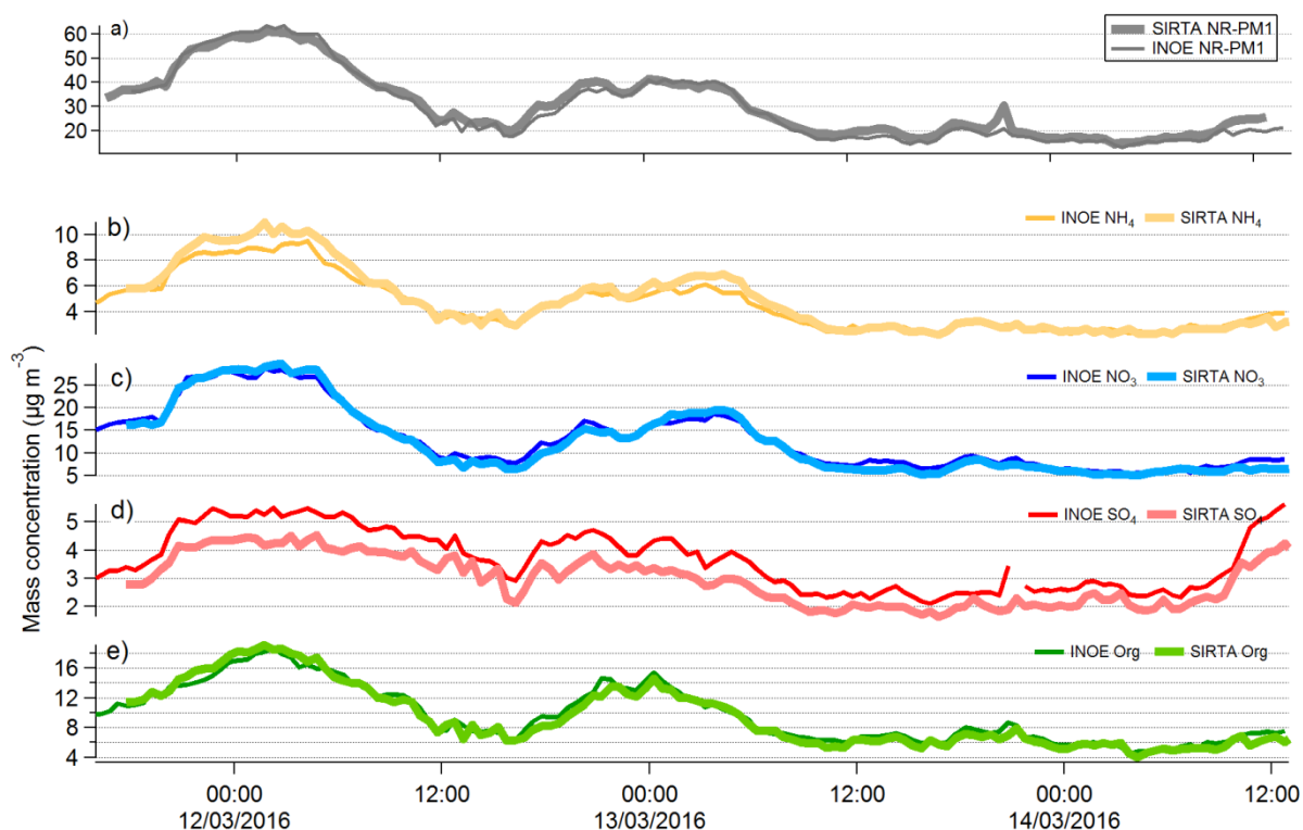
Figure 5.1. Comparison of INOE instrument with the reference instrument for a) Total PM, b) Ammonia, c) Nitrate, d) sulphate, and e) Organic.
