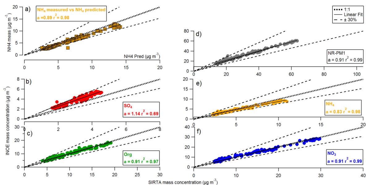
Figure 5.2. a) \text{NH}_4 measured vs \text{NH}_4 predicted for INOE instrument, and comparison of the INOE instrument with the Sirta instrument for b) \text{SO}_4 , c) Org, d) Total NR-PM1 mass concentration, e) \text{NH}_4 , and f) \text{NO}_3 .
