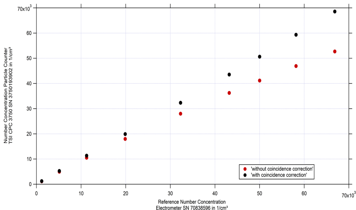
Fig. 2: Linearity test for TSI CPC 3750 SN 3750193902 against aerosol electrometer 3068 SN 70838596; silver particles with a diameter of 30 nm were used for number concentrations between 1000 and 70000 particles per cm^3 .
