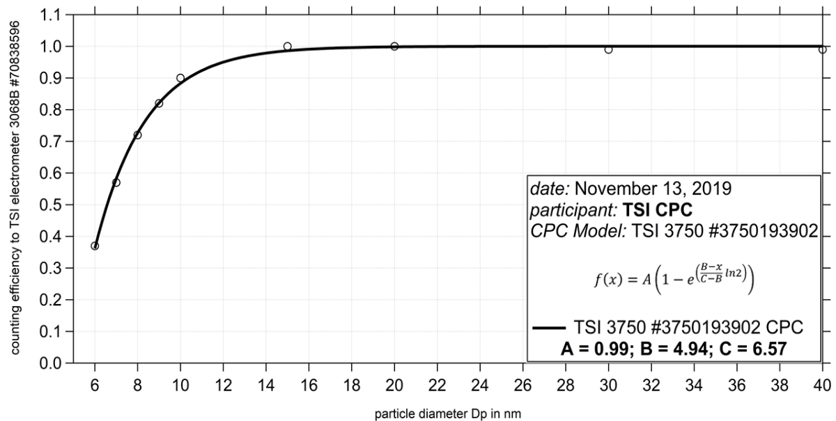
Fig. 1: Counting efficiency for CPC 3750 S/N 3750193902 against aerosol electrometer 3068 S/N 70838596; silver particles between 6 and 40 nm were used for calibration; the calculated D_{p50} is 6.57 nm.
