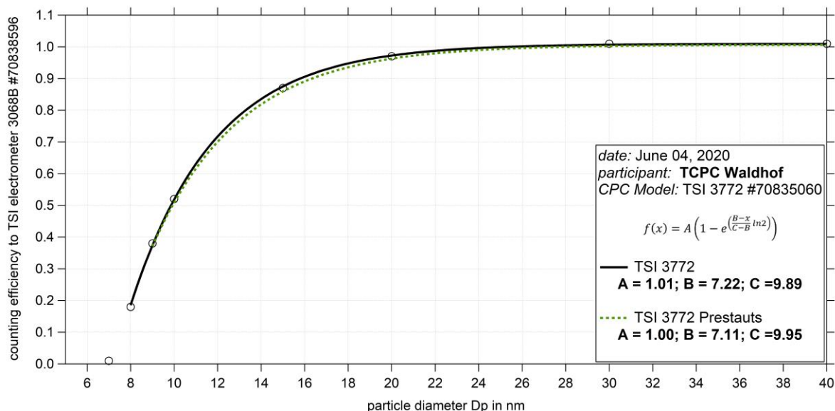
Fig. 1: Counting efficiency for Total CPC 3772 S/N 70835060 against aerosol electrometer 3068 S/N 70838596; silver particles between 7 and 40 nm were used for calibration; The instrument was calibrated to Dp50 of 10nm and resulted in a Dp50 of 9.89nm. The graph shows the counting efficiency before the calibration and after.
