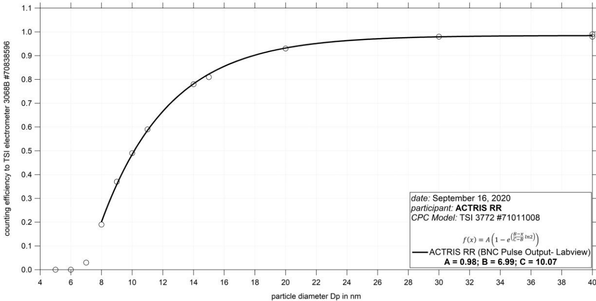
Fig. 1: Counting efficiency for CPC 3772 S/N 71011008 against aerosol electrometer 3068 S/N 70838596; silver particles between 5 and 40 nm were used for calibration.
