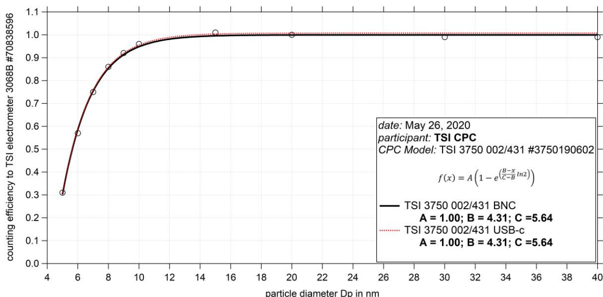
Fig. 1: Counting efficiency for CPC 3750 002/431 S/N 3750190602 against aerosol electrometer 3068 S/N 70838596; silver particles between 5 and 40 nm were used for calibration; the calculated Dp50 is 5.64 nm.
