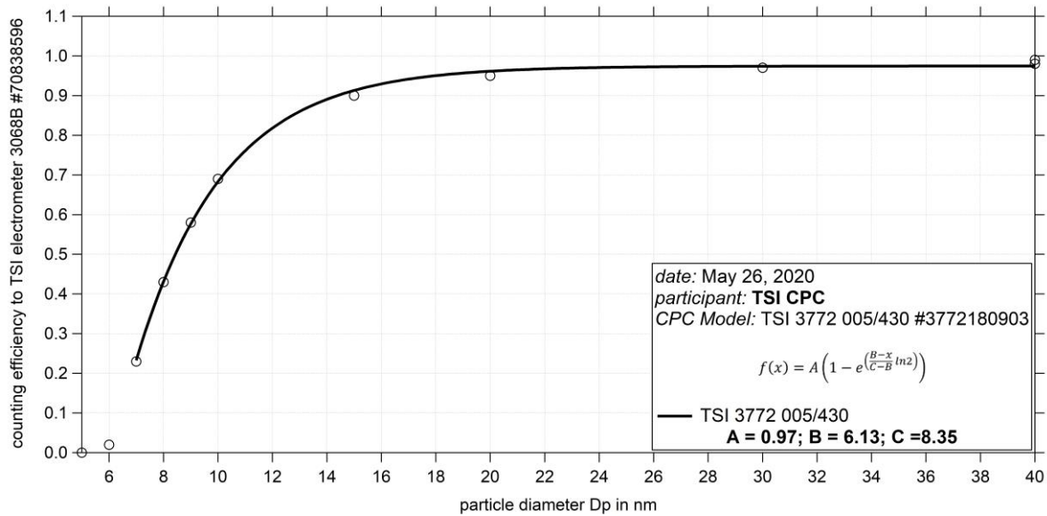
Fig. 1: Counting efficiency for CPC 3772 005/430 S/N 3772180903 against aerosol electrometer 3068 S/N 70838596; silver particles between 5 and 40 nm were used for calibration; the calculated D_{p50} is 8.35 nm.
