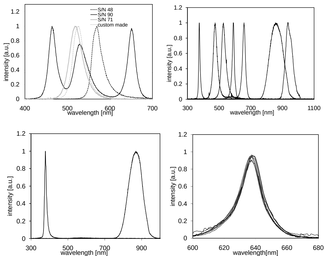
Fig. 4. Normalized spectral emission of light sources of absorption photometers. (a) different types of PSAPs; single wavelength Radiance Research PSAPs (S/N 48, S/N 71); three wavelength Radiance Research PSAP (S/N 90); custom made (ITM). (b) seven wavelength Aethalometer model AE31 (S/N 563). (c) two wavelength Aethalometer model AE21 (S/N 426) and (d) seven MAAPs.
