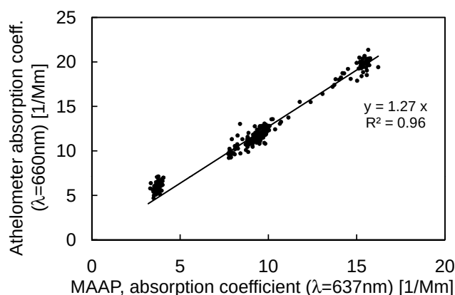
Fig. 8. Ambient air runs during GAW2005. Aethalometer (model AE31, 660 nm) absorption coefficient vs. MAAP absorption coefficient ( \lambda = 637 nm). Aethalometer data were corrected using Weingartner et al. (2003).
