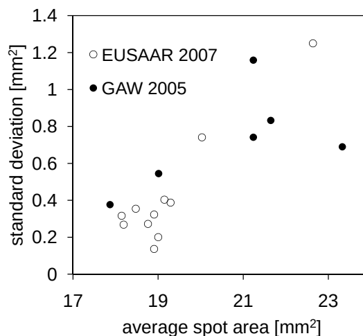
Fig. 5. Standard deviation of PSAP spot area versus average spot area. Each point is for one PSAP. The nominal spot area given by the manufacturer is 17.85 mm 2 .
